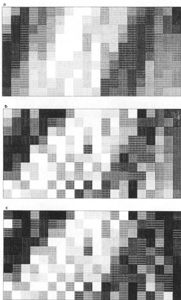
FIG. 8. The influence of 50% noise on the solutions for wide-angle illumination. (a) SVD for 40 eigenvectors, misfit 0.284, (b) undamped Paige-Saunders solution after 5 iterations, misfit 0.254, and (c) Dines-Lytle after 20 iterations, misfit 0.237.
