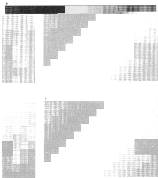
FIG. 5. Paige-Saunders solution for wide-angle illumination; (a) undamped solution after 20 iterations, misfit 0.007, and (b) after convergence to almost machine precision in 400 iterations.
