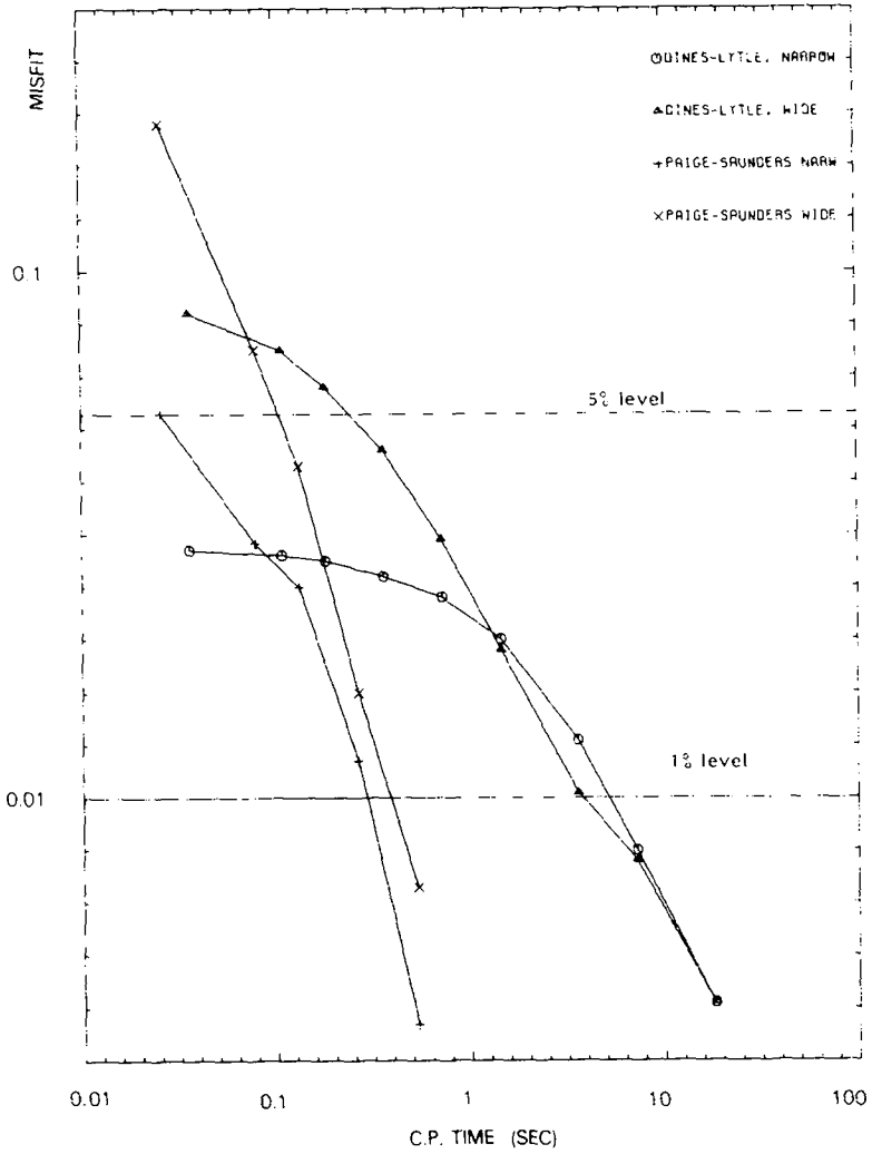
FIG. 7. Decrease of the normalized length of the residual vector as a function of central processor
